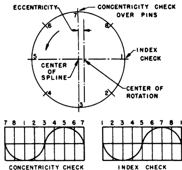
FIG. 29—INDEX READINGS DUE TO ECCENTRICITY
