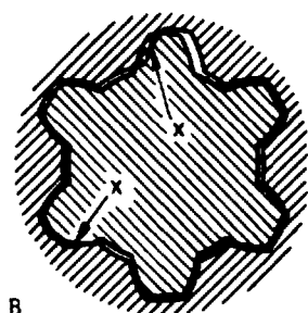
THE PERFECT EXTERNAL SPLINE WITH BASIC TOOTH THICKNESS INTERFERES AT X.
