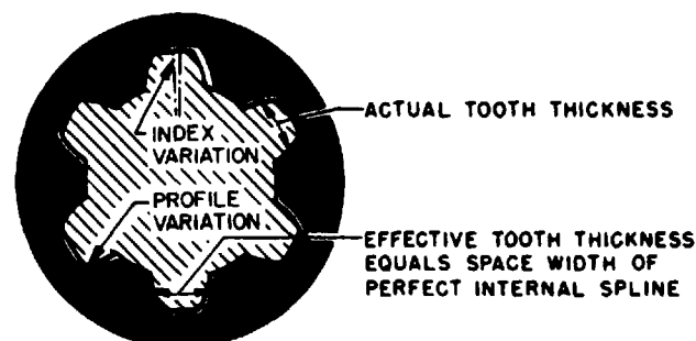
THE PERFECT INTERNAL SPLINE FITS IN ANY POSITION, IF ALL TEETH OF THE EXTERNAL ARE NARROWED BY THE AMOUNT OF THE INTERFERENCE.
