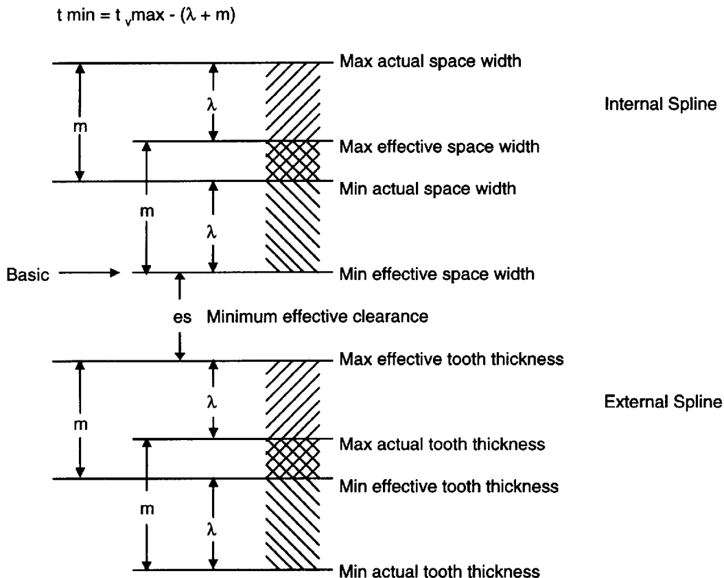
Figure 1. Tooth thickness, space width, and minimum effective clearance
