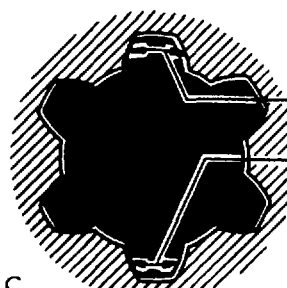
THE PERFECT EXTERNAL SPLINE FITS IN ANY POSITION, IF ALL SPACES ARE WIDENED BY THE AMOUNT OF THE INTERFERENCE.
