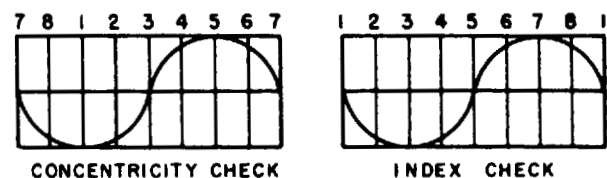
FIG. 29—INDEX READINGS DUE TO ECCENTRICITY
