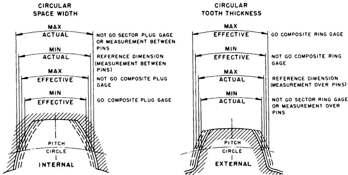
FIG. 11—SPACE WIDTH AND TOOTH THICKNESS INSPECTION
