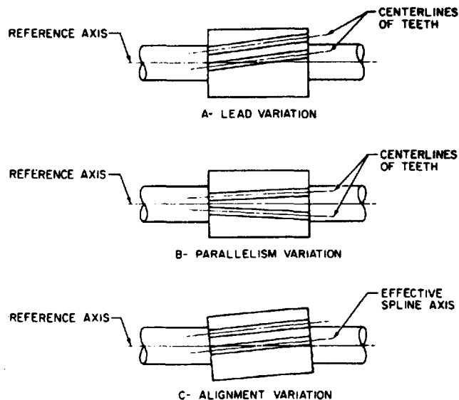
FIG. 1—LEAD VARIATIONS
