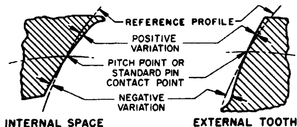
FIG. 2—PROFILE VARIATIONS
