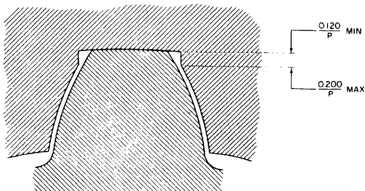
FIG. 34—INTERNAL CORNER CLEARANCE
