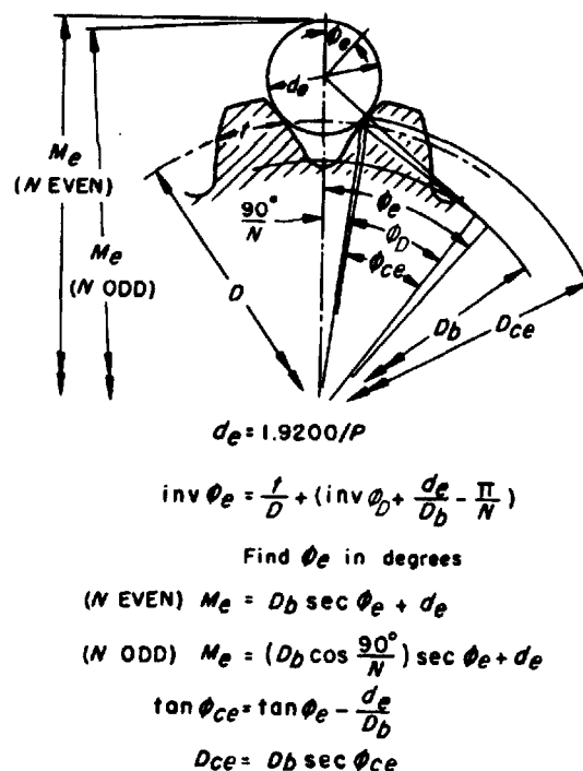
FIG. 25—MEASUREMENT OVER PINS OF EXTERNAL INVOLUTE SPLINES
