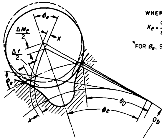
FIG. 38—MEASUREMENT CHANGE FACTOR K_e FOR EXTERNAL SPLINES
