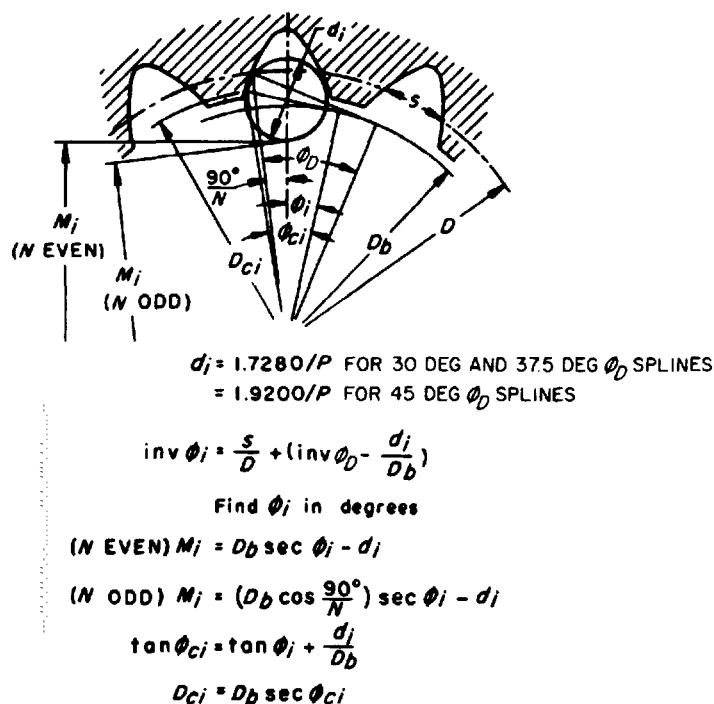
FIG. 23—MEASUREMENT BETWEEN PINS OF INTERNAL INVOLUTE SPLINES
