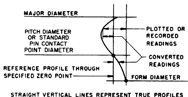
FIG. 32—ANALYSIS OF PROFILE READINGS
