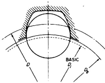
FIG. 26—SIX-TOOTH INTERNAL SPLINE
