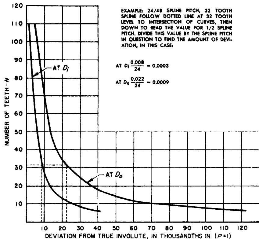
FIG. 10B—DEVIATION FROM TRUE INVOLUTE OF INTERNAL STRAIGHT SIDED 45 DEG PRESSURE ANGLE SPLINES
