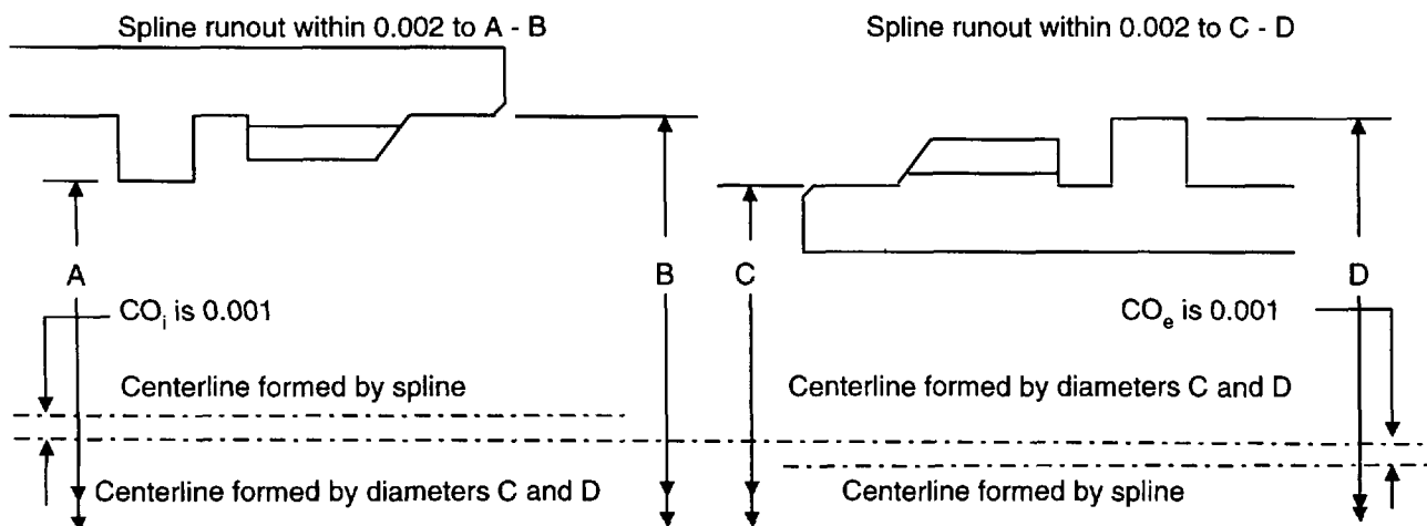
Figure 2. Sample calculation for eccentricity
