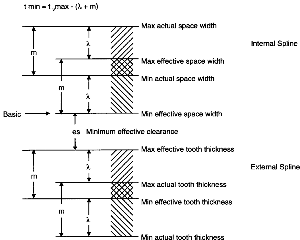
Figure 1. Tooth thickness, space width, and minimum effective clearance
