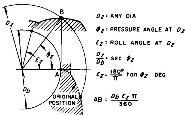
FIG. 31—USE OF ROLL ANGLES
