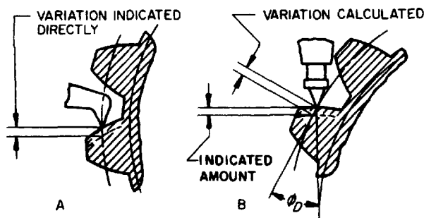
FIG. 33—INDICATING LEAD VARIATION
