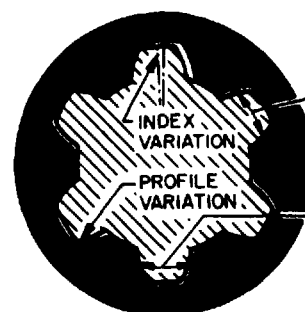
C THE PERFECT INTERNAL SPLINE FITS IN ANY POSITION, IF ALL TEETH OF THE EXTERNAL ARE NARROWED BY THE AMOUNT OF THE INTERFERENCE.
