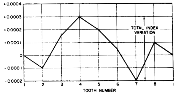
FIG. 28—INDEX VARIATION CHART
