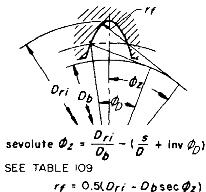
FIG. 35—FILLET FOR FILLET ROOT INTERNAL SPLINE
