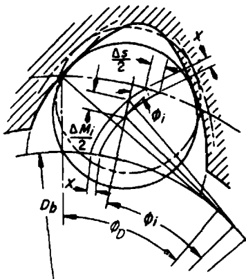
FIG. 37—MEASUREMENT CHANGE FACTOR K_i FOR INTERNAL SPLINES
