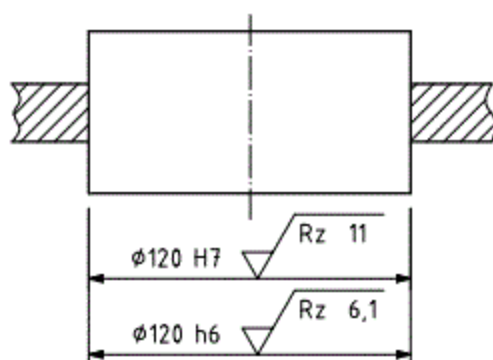
Figure 19 — Surface texture requirement — Feature-of-size dimension
