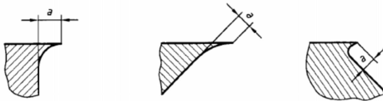
Figure 2 — States of an internal edge
