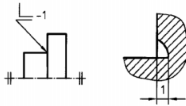
Figure 12 — Direction of the undercut on an internal edge
