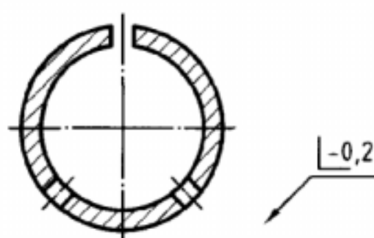
Figure 17 — State of edge common to all the edges of a part
