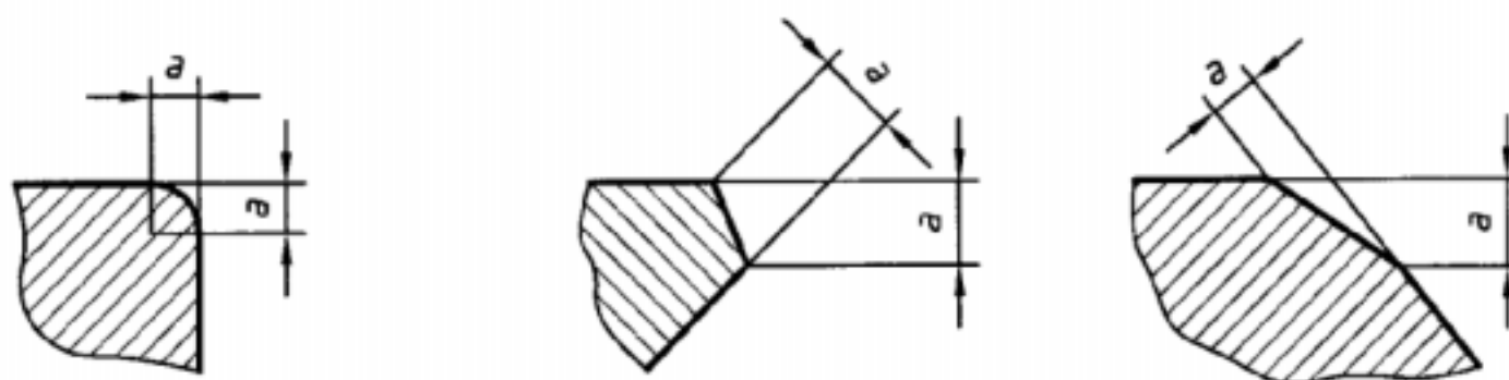
Figure 3 — Examples of burr
