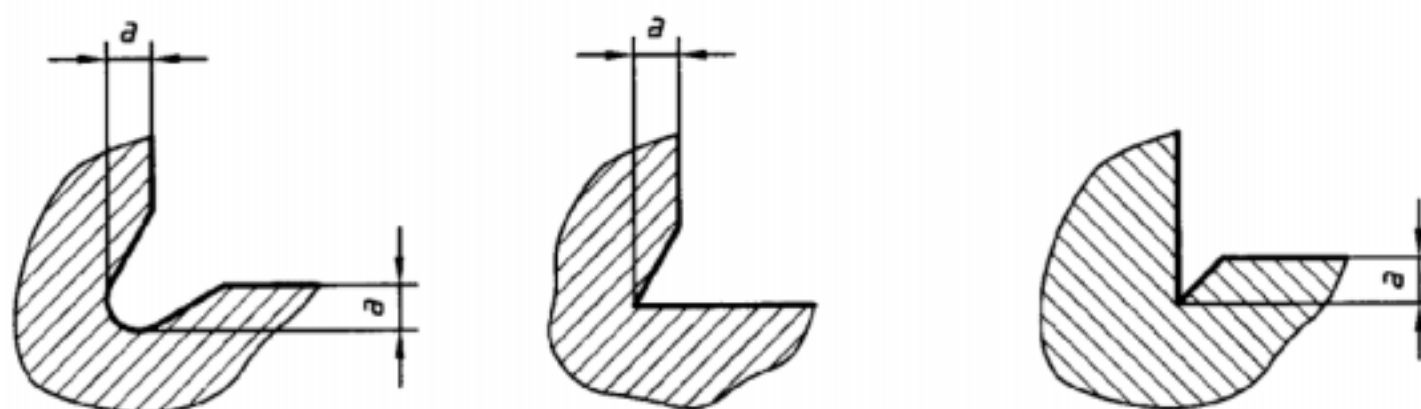
Figure 4 — Examples of undercut at an external edge
