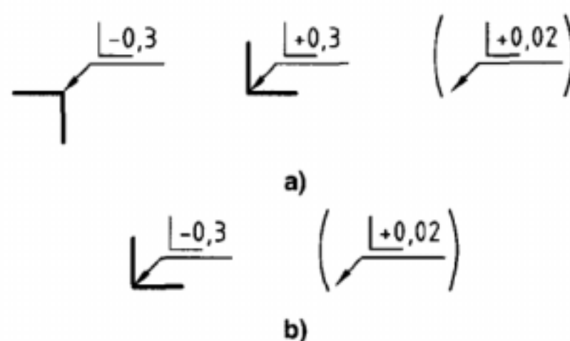
Figure 20 — Additional states of edges in the context of a collective indication
