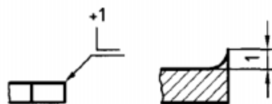
Figure 11 — Direction of the burr on an external edge
